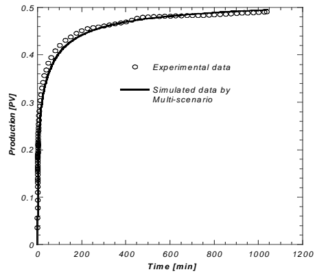
Figure 12: Reconciliation of the single-speed centrifuge experiment.
