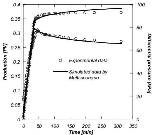
Figure 17: Reconciliation of the unsteady state experiment by the multi-scenario feature.
