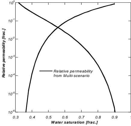
Figure 10: Estimated relative permeabilities using the multi-scenario feature.
