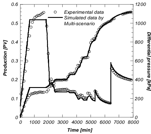
Figure 13: Reconciliation of the steady state experiment.
