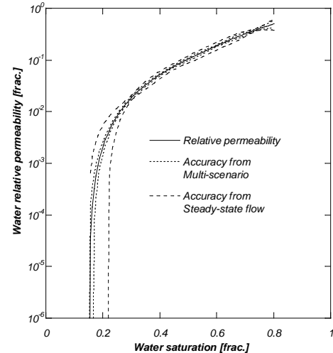
Figure 5: Water relative permeability from steady state data and multi-scenario estimation.
