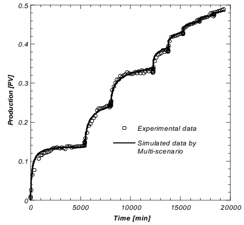
Figure 14: Reconciliation of the multi speed centrifuge experiment.
