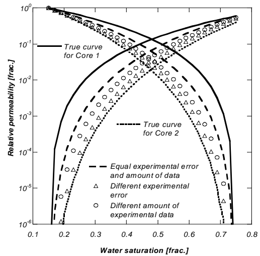
Figure 9: True and estimated relative permeability curves.
