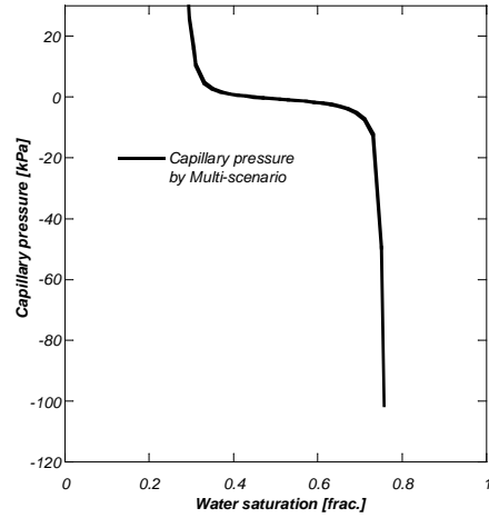
Figure 16: Estimated capillary pressure using the multi-scenario feature, Extended Corey and Brooks representation.
