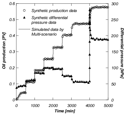
Figure 2: Reconciliation of the steady state data.
