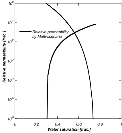
Figure 15: Estimated relative permeabilities using the multi-scenario feature, Corey representation.
