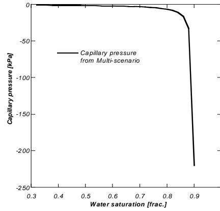
Figure 11: Estimated capillary pressure using the multi-scenario feature.
