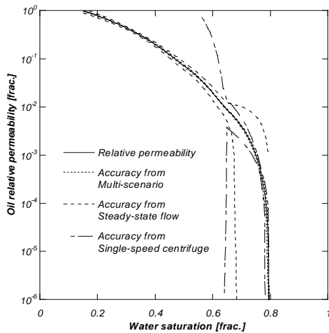
Figure 6: Oil relative permeability from steady state data, single speed centrifuge data.
