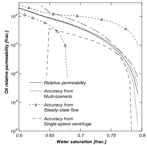
Figure 7: Oil relative permeability at high water saturations, magnification of Figure 6.
