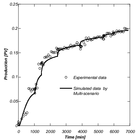
Figure 18: Reconciliation of the multi speed centrifuge experiment.
