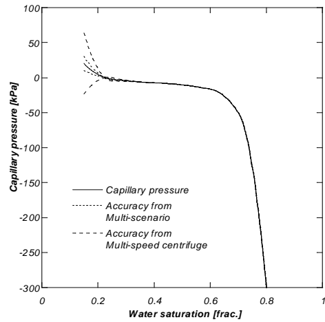
Figure 8: Capillary pressure from multi speed centrifuge data and multi scenario estimation.
