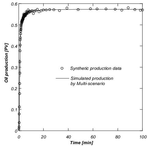
Figure 3: Reconciliation of the single speed centrifuge data.
