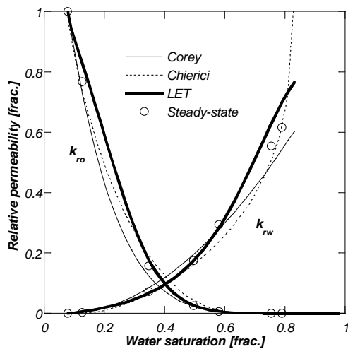
Figure 7: Relative permeability; linlin.
