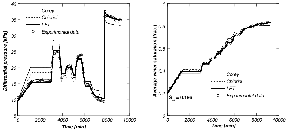
Figure 1: History match of differential pressure Figure 2: History match of production
