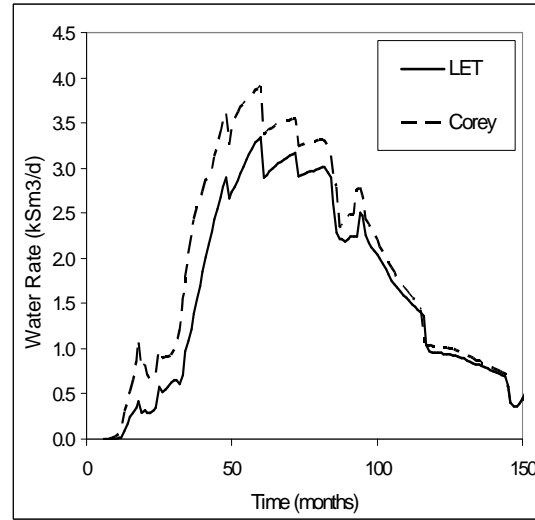
Figure 10: Water production rate of a sector
