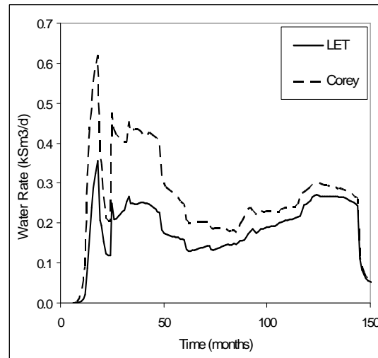
Figure 12: Water production rate of a well
